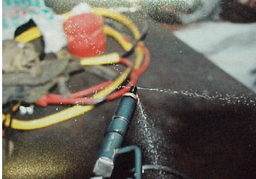
Figure 3: Poor injector spray pattern
