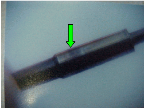
Figure 5: Arrow indicates scratches on needle shank
