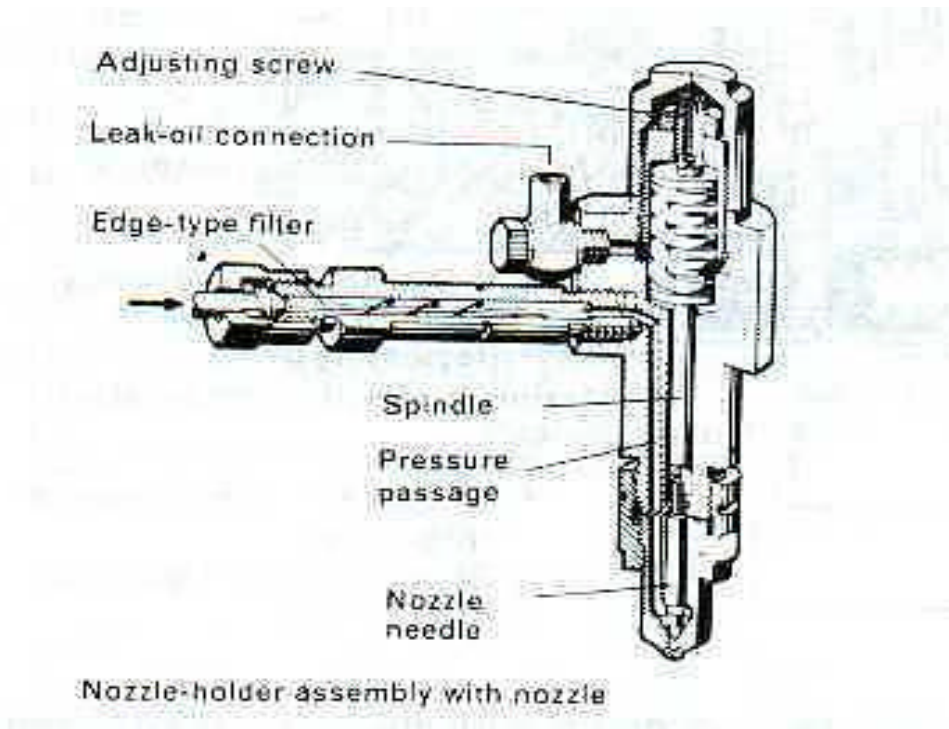
Figure 7: Injector layout
